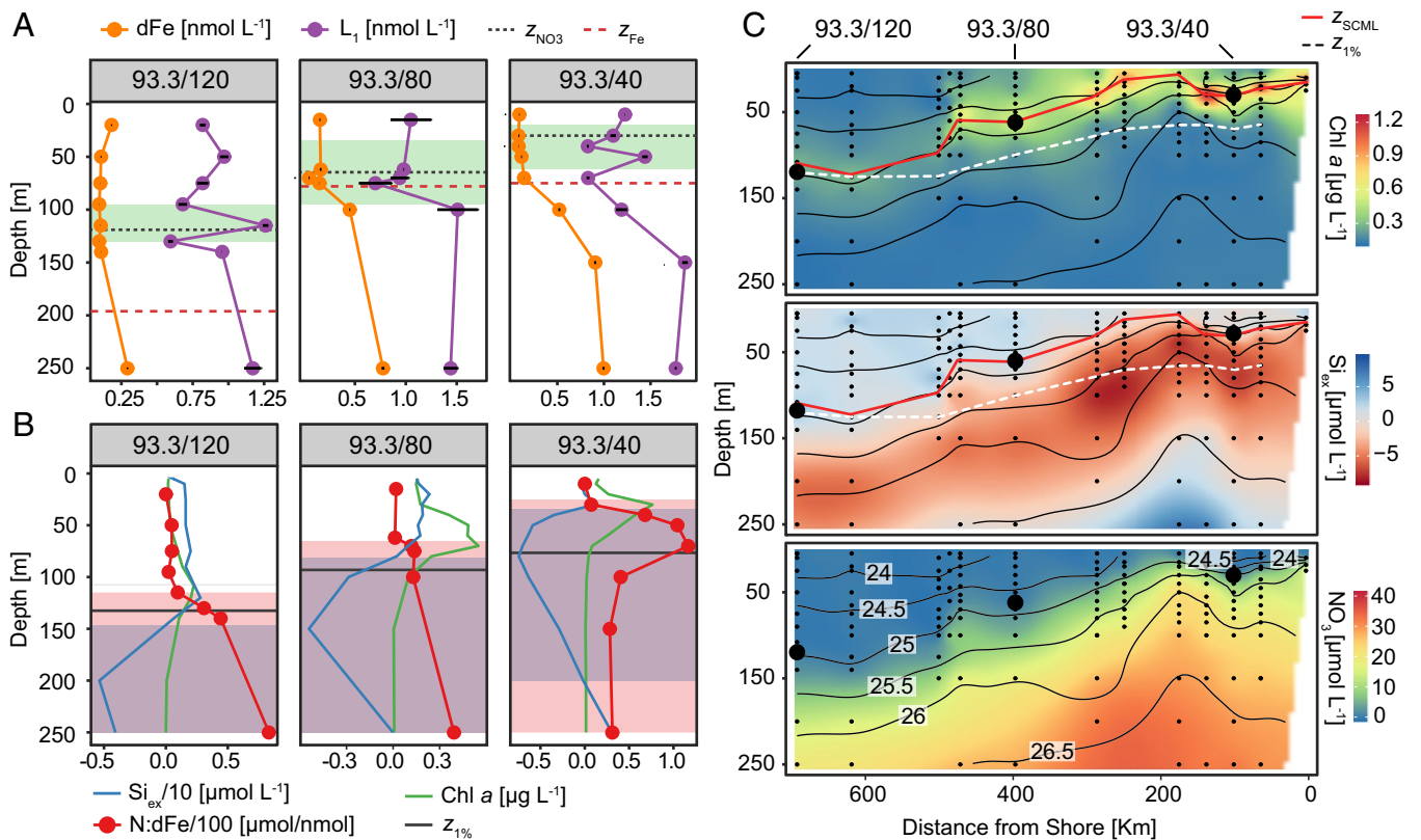
Fig. 1. (A) Profiles of dissolved Fe (orange) and L_1 (purple) concentrations. The green box denotes depths where chlorophyll a (Chl a ) is within 50% of the concentration at the SCML depth ( z_{SCML} ), the dashed black line is nitracline depth ( z_{NO_3} ), and the dashed red line is ferricline depth ( z_{Fe} ) (SI Appendix, Table S1 and section 4). (B) Profiles of Chl a (green), Si_{ex}/10 (blue), and N:dFe/100 (red). The black line represents the depth of 1% of incident irradiance ( z_{1\%} ). Red ( N:dFe \geq 8 ), blue ( Si_{ex} < 0 ), and purple (both proxies) indicate depth ranges with potential diatom Fe deficiency. (C) Chl a , NO_3 , and Si_{ex} ( 26.5 \text{ kg} \cdot \text{m}^{-3} source isopycnal) sections. Potential density anomaly ( \sigma_\theta ) contours are in black. Small circles show nutrient sampling depths and large circles show incubation and metatranscriptome depths. White and red dashed lines show z_{1\%} and z_{SCML} , respectively.
